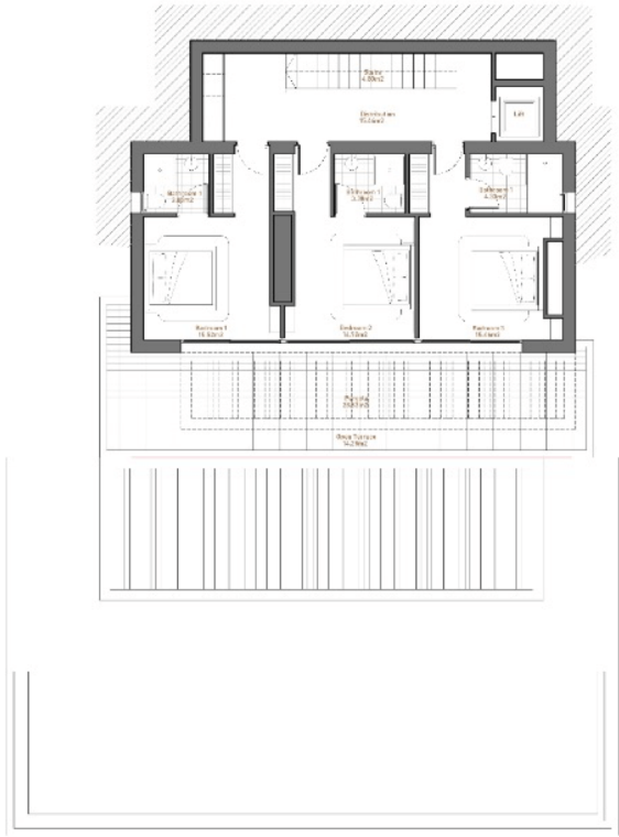
LEVEL +155.20 (Bedrooms) BUILT AREA Living area 102.84m 2 Veranda 23.83m 2 Open Terrace 18.74m 2
