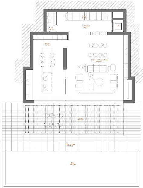
LEVEL +151.80 (Ground Floor - Living) BUILT AREA Living area 145.42m 2 Veranda 48.35m 2 Open Terrace 51.27m 2 Pool 54.00m 2
