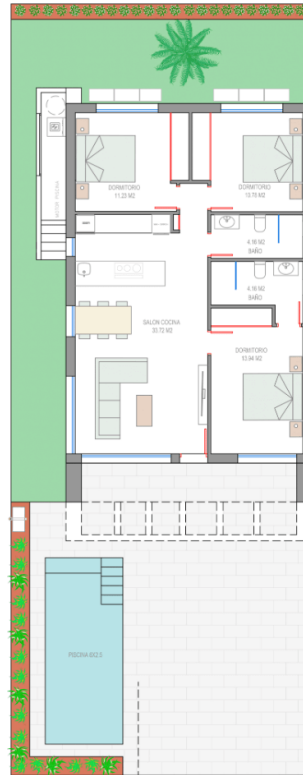
VILLAS 12-21 VILLA SQUARE 109m 2 PLOT 246m 2
