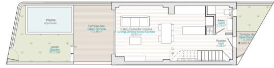
Planta 1 | Floor 1
