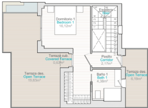
Planta 1 | Floor 1
